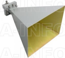
LB-159-20-C-TF Standard Gain Horn Antenna 4.9-7.05GHz 20dB Gain TNC Female
