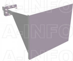
LB-159-20-C-SFSPO Standard Gain Horn Antenna 4.9-7.05GHz 20dB Gain SMA Female
